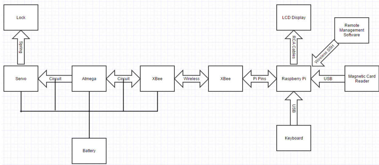
Figure 2, Block Diagram of Project with Interconnections
